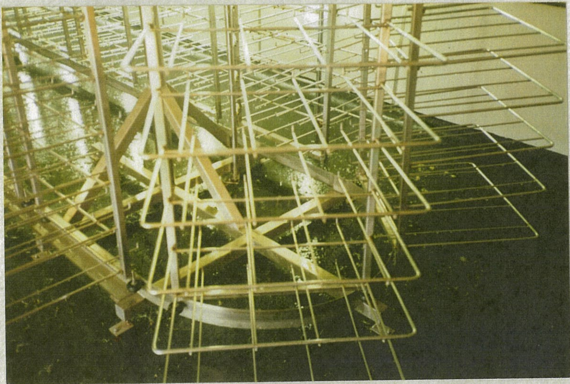
Jan 1988 Shows construction of our own design Rotary tray system.
